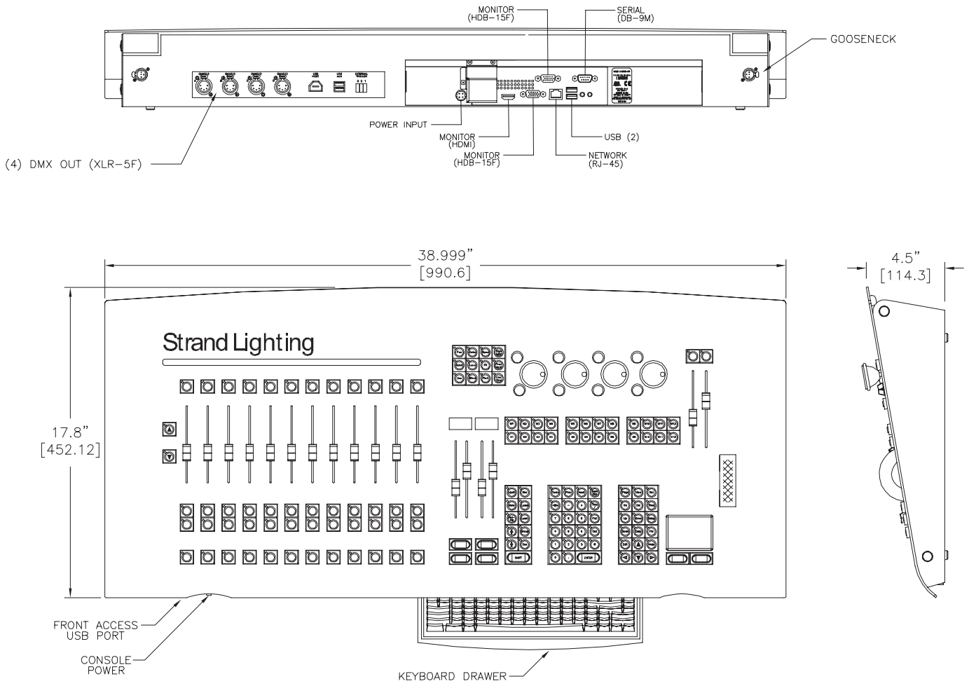
Light Palette Classic Lighting Control Console
