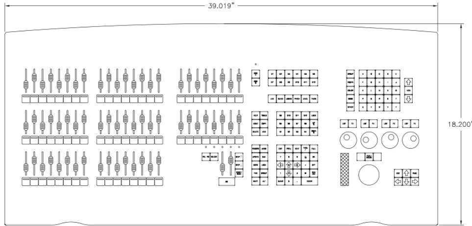
92816 • Palette VL 1500 Channel, 64 submaster console
