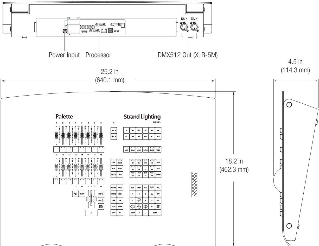
92800 Basic Palette II Memory Console with 100 Channels, 16 Submasters
