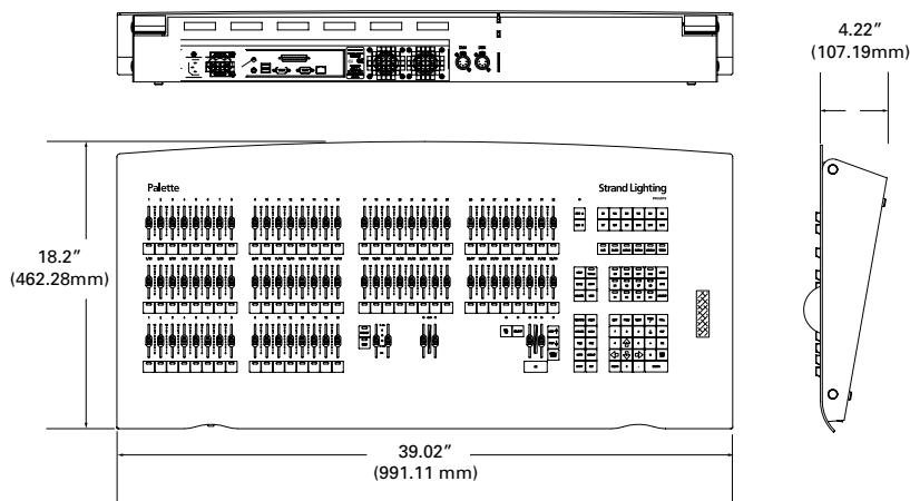
92801 preset Palette II Memory-Manual Console 32/64 with 100 channels
