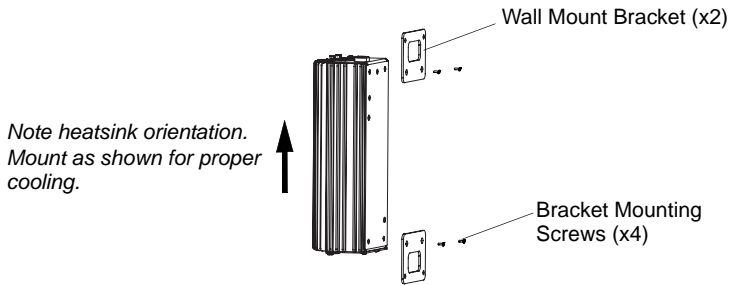
Figure 2: LightPack LED Module Wall Mounting
