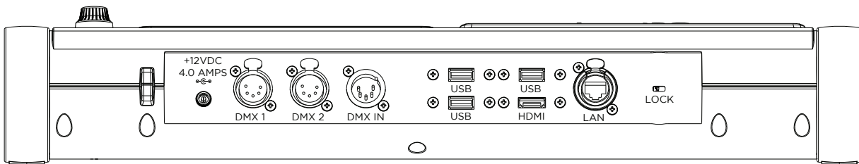
FIGURE 2. CONNECTIONS
