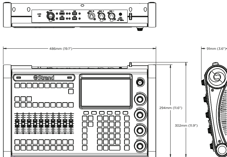
FIGURE 3. DIMENSIONS
