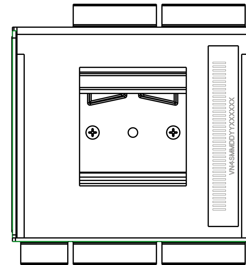
DIN RAIL MOUNT CONFIGURATION (AS SHIPPED)
