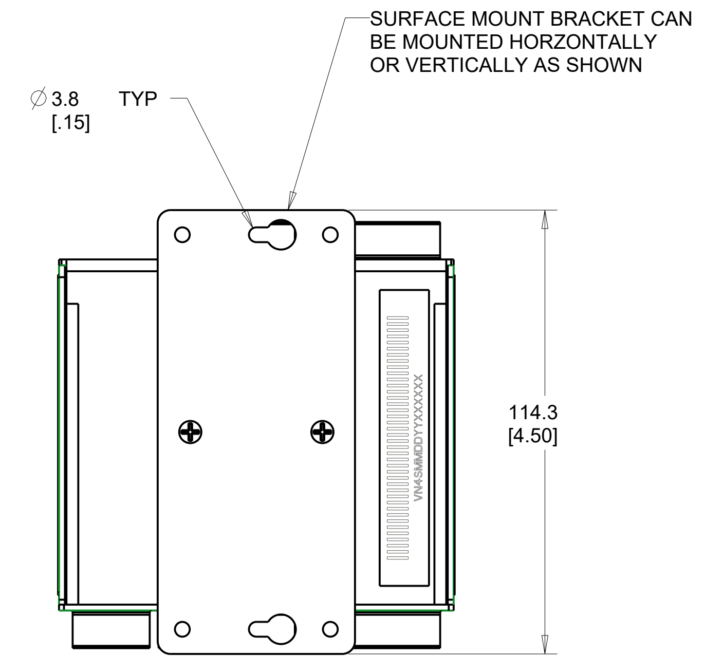
SURFACE MOUNT CONFIGURATION
